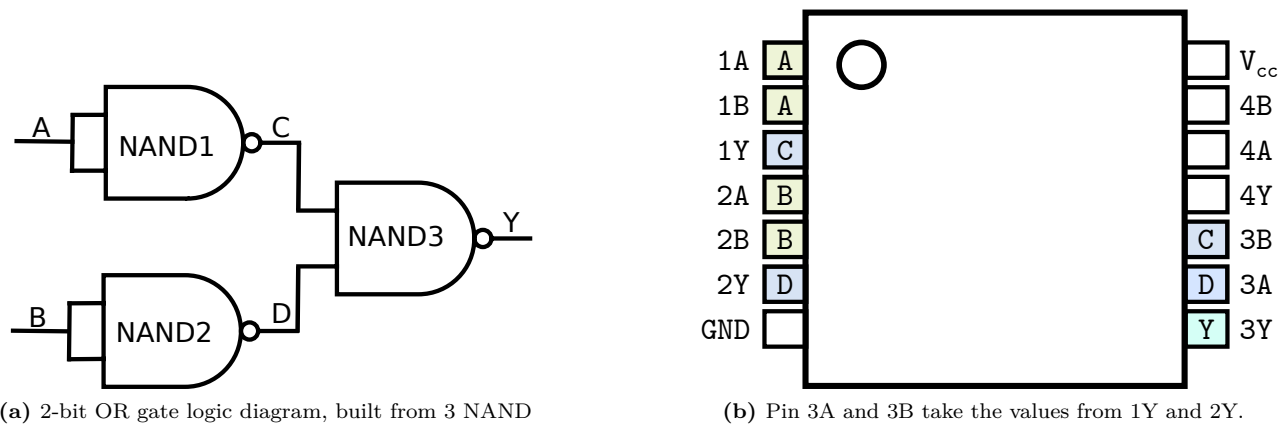
Figure 2.3.3: 2-bit OR gate implementation
