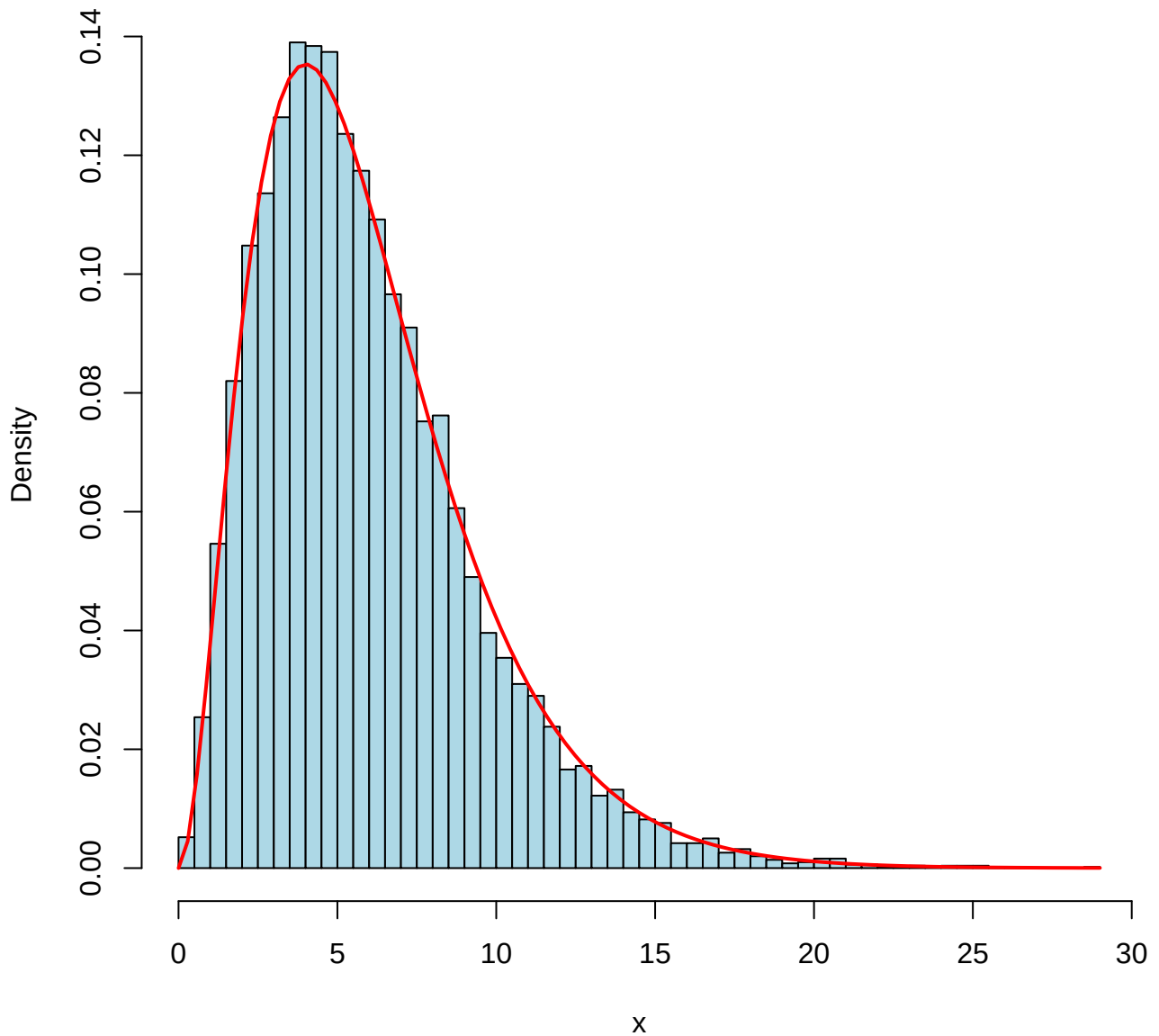
Chi-square Distribution (df = 6 )
