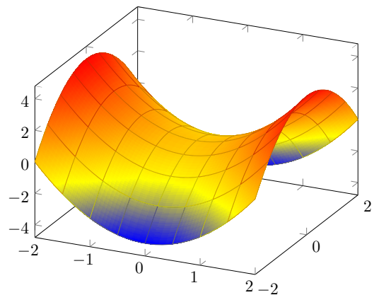
Figure 1. Hyperbolic paraboloid obtained from PGFPlots [PFGPlots].
