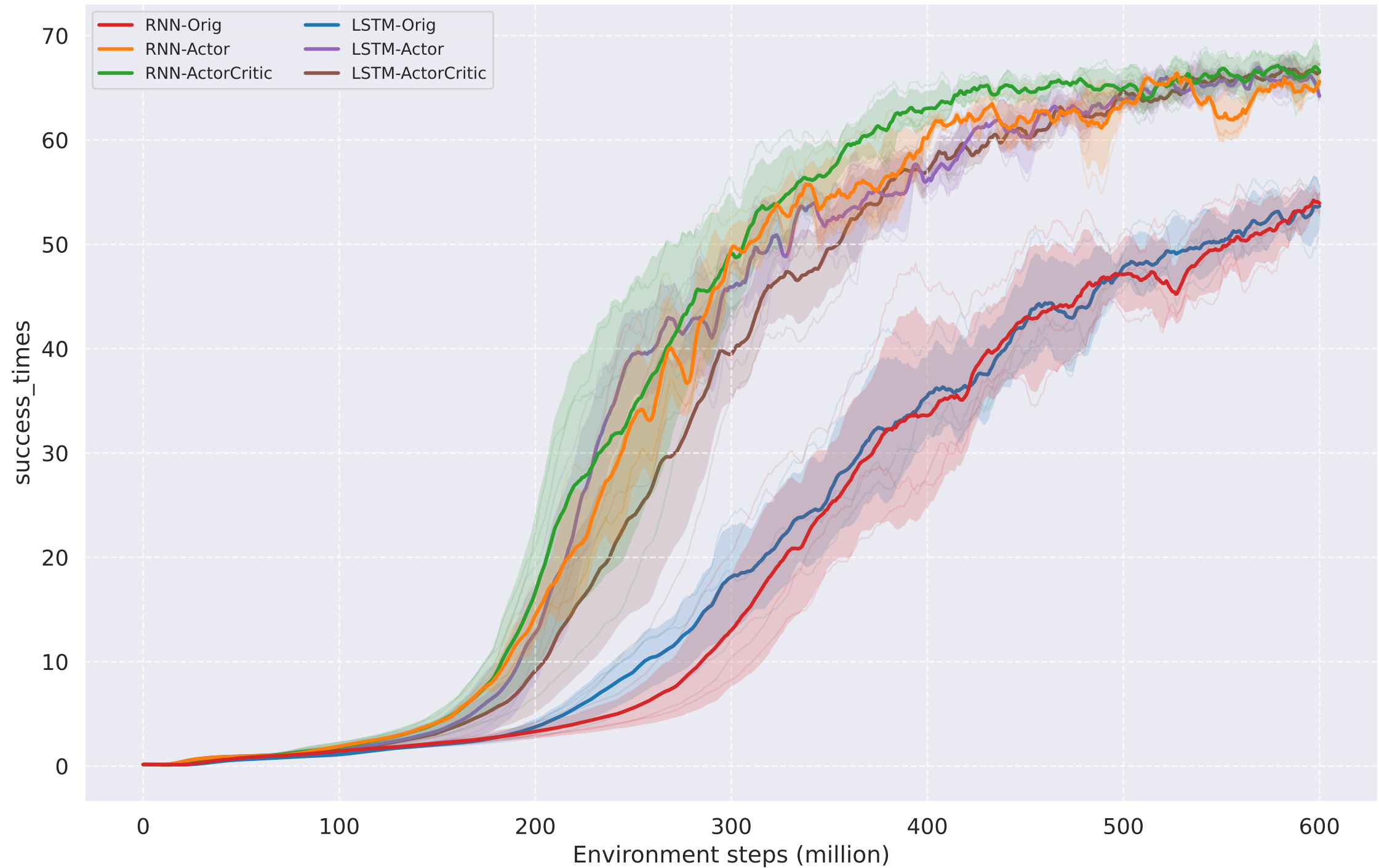
RNN vs LSTM (6 variants) performance: eval/success_times
