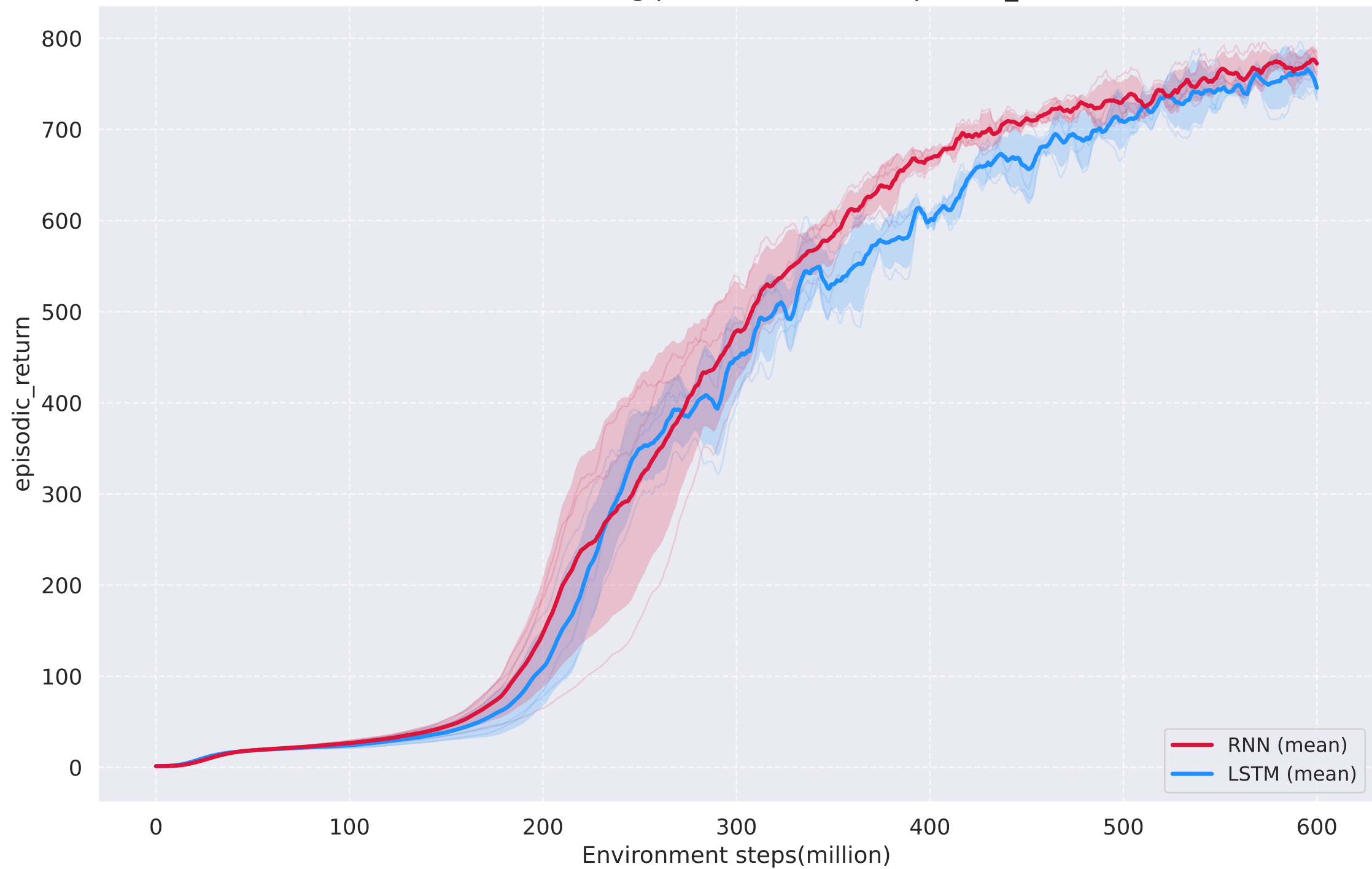
RNN vs LSTM training performance(eval/episodic_return)
