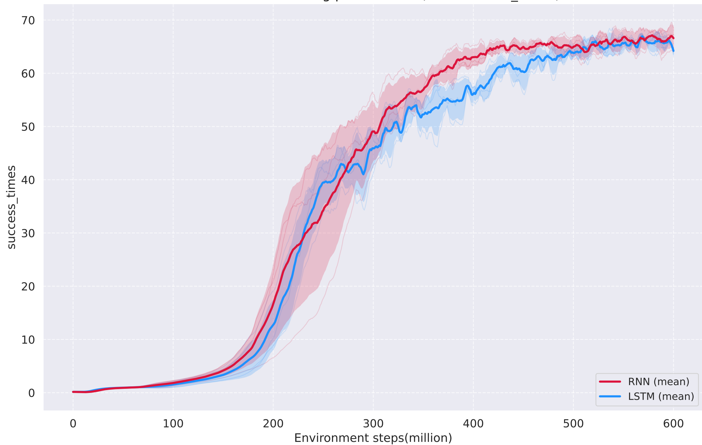
RNN vs LSTM training performance(eval/success_times)
