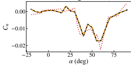
C_n (Yawing Moment)
