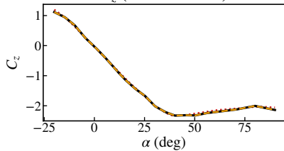
C_z (Normal Force)
