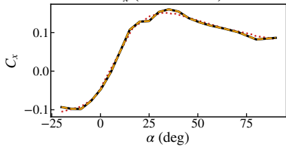
C_x (Axial Force)
