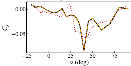
C_y (Side Force)
