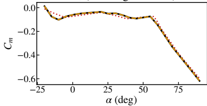
C_m (Pitching Moment)
