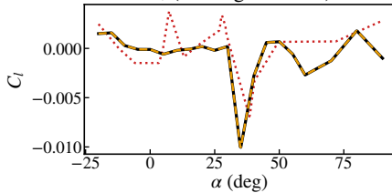
C_l (Rolling Moment)
