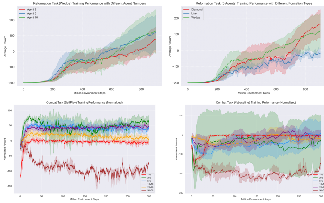
Fig. 6. Learning Curves across Benchmark Tasks. (Top) IPPO training returns for the decentralized formation keeping task across varying swarm sizes ( N = 2, 5, 10 ) and geometric templates (Wedge, Diamond, Line). (Bottom) Hierarchical MAPPO returns in the adversarial pursuit-evasion benchmark under self-play and fixed-baseline settings, demonstrating successful convergence from 1-vs-1 up to massive 50-vs-50 engagements. Shaded regions denote the standard error across multiple random seeds.
