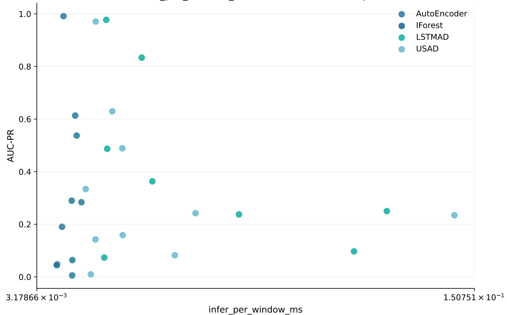
Pareto: AUC-PR vs infer_per_window_ms (mean across seeds per (model, dataset))
