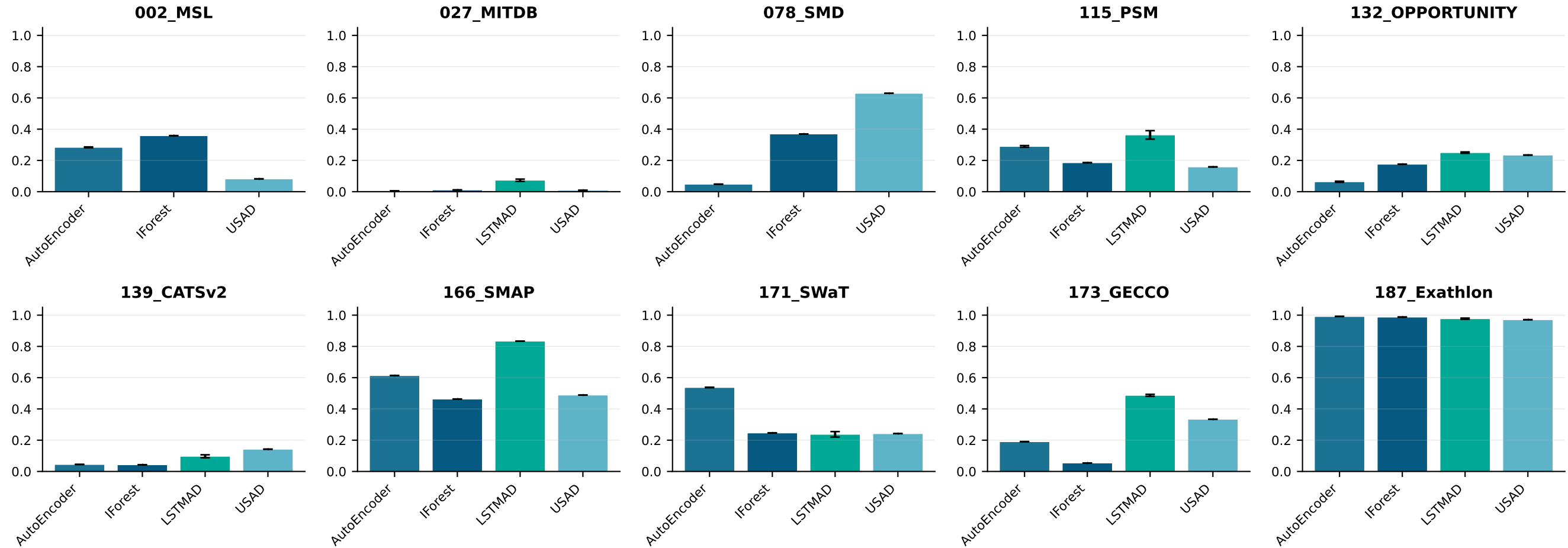
AUC-PR per dataset (error bars = \pm 1 SD across seeds)
