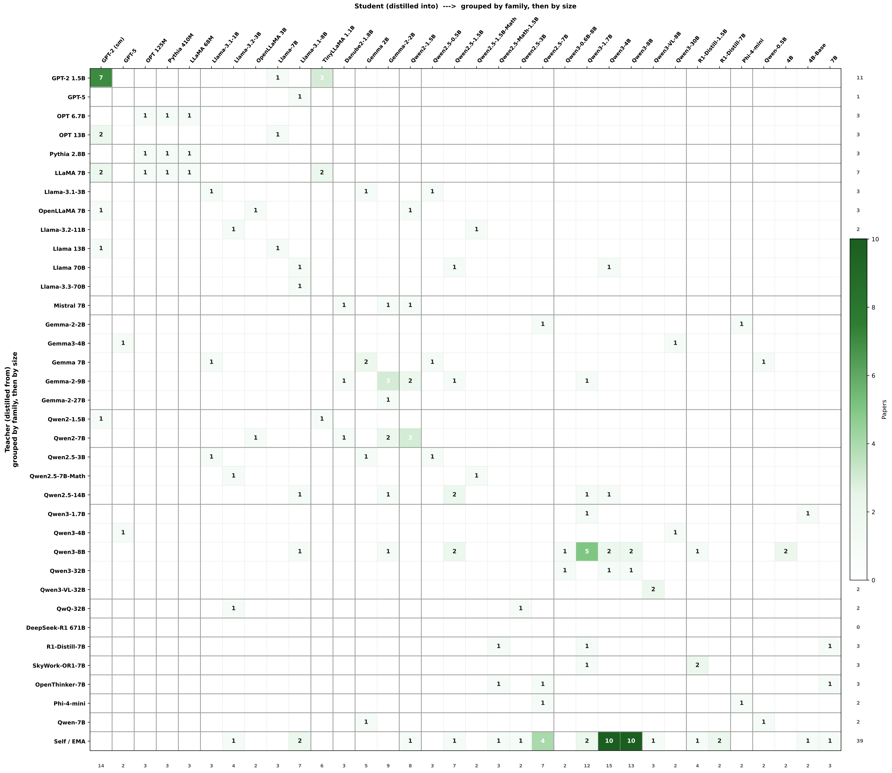
On-Policy Distillation: Teacher x Student Pair Matrix (119 papers) Cell = number of papers using that (teacher -> student) combination
