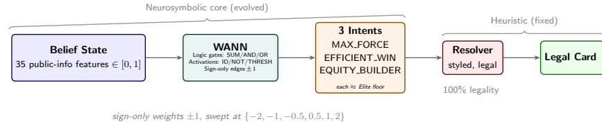
Fig. 1. The Sueca-WANN pipeline. A 35-feature public-information belief state feeds a weight-agnostic neural network built from logic gates (SUM/AND/OR aggregations; IDENTITY/NOT/THRESHOLD activations), which outputs three play intents. A fixed, hand-authored styled resolver maps the selected intent to a legal card. The neurosymbolic core (belief \rightarrow WANN \rightarrow intents) is evolved; the resolver is a deterministic heuristic guaranteeing 100% legality.
