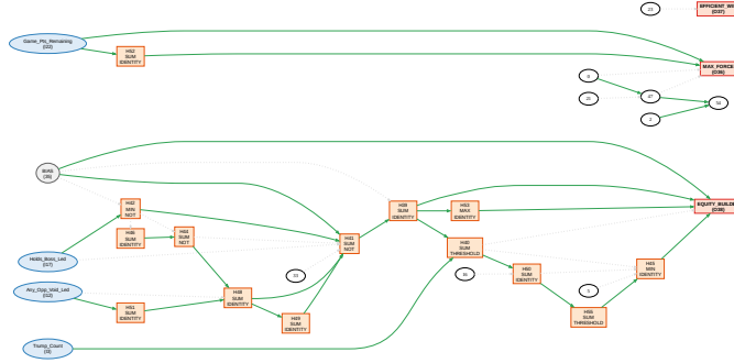
Fig. 3. The v6 champion’s follow-brain topology before minification (17 hidden gates, 44 connections). After constant-folding and alias inlining, the active logic reduces to 5 gates at depth 5 (see Listing 1.1).
