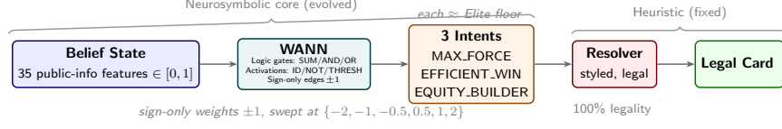
Fig. 1. The Sueca-WANN pipeline. A 35-feature public-information belief state feeds a weight-agnostic neural network built from logic gates (SUM/AND/OR aggregations; IDENTITY/NOT/THRESHOLD activations), which outputs three play intents. A fixed, hand-authored styled resolver maps the selected intent to a legal card. The neurosymbolic core (belief \rightarrow WANN \rightarrow intents) is evolved; the resolver is a deterministic heuristic guaranteeing 100% legality.
