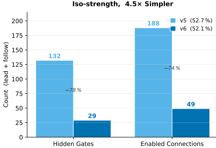
Fig. 6. Complexity comparison: v5 champion (alpha-beta teacher, 132 hidden gates) vs. v6 champion (rollout teacher, 29 gates). Iso-strength, 4.5× simpler.
