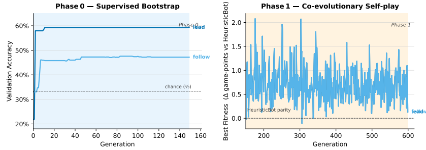
Fig. 2. Training curves for the v6 champion. Phase 0 (generations 0–149): supervised classification accuracy on lead and follow dataset splits, starting from zero connections. Phase 1 (generations 150–599): co-evolutionary self-play fitness (game-point delta vs. HeuristicBot). The Phase 0→1 transition re-evaluates HOF entries under Phase 1 fitness.
