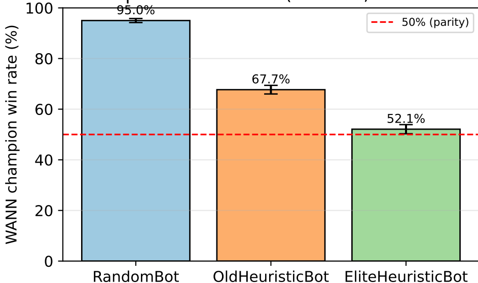
v6 champion vs baselines (n=3000, seat-rotated)
