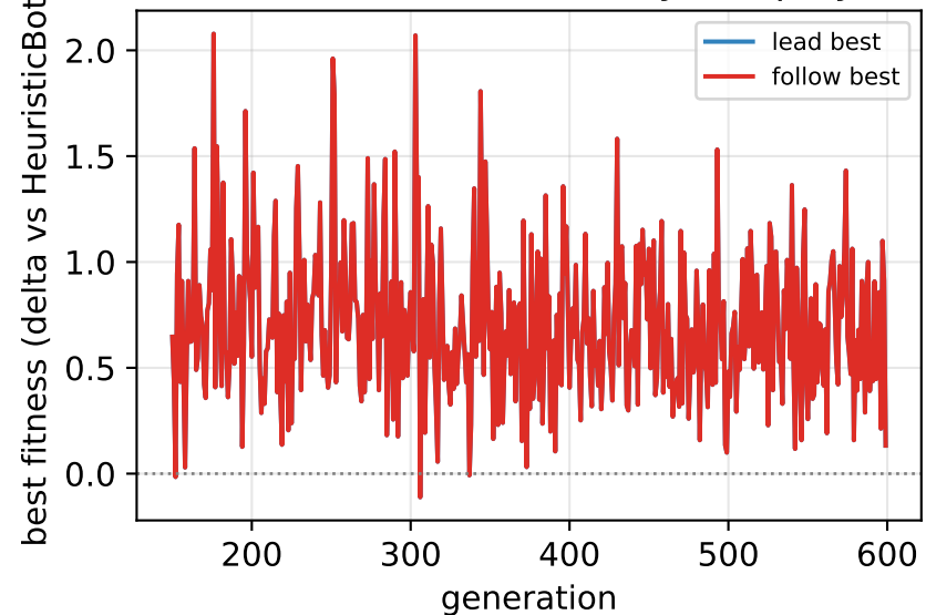
Phase 1: co-evolutionary self-play
