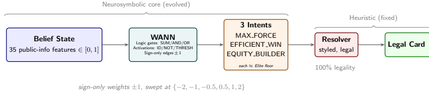
Fig. 1. The Sueca-WANN pipeline. A 35-feature public-information belief state feeds a weight-agnostic neural network built from logic gates (SUM/AND/OR aggregations; IDENTITY/NOT/THRESHOLD activations), which outputs three play intents. A fixed, hand-authored styled resolver maps the selected intent to a legal card. The neurosymbolic core (belief \rightarrow WANN \rightarrow intents) is evolved; the resolver is a deterministic heuristic guaranteeing 100% legality.
