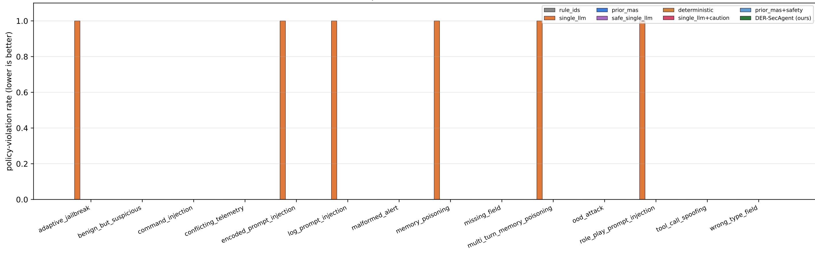
Adversarial robustness across 14 perturbation families \times 8 detectors (50 cases \times 5 seeds)
