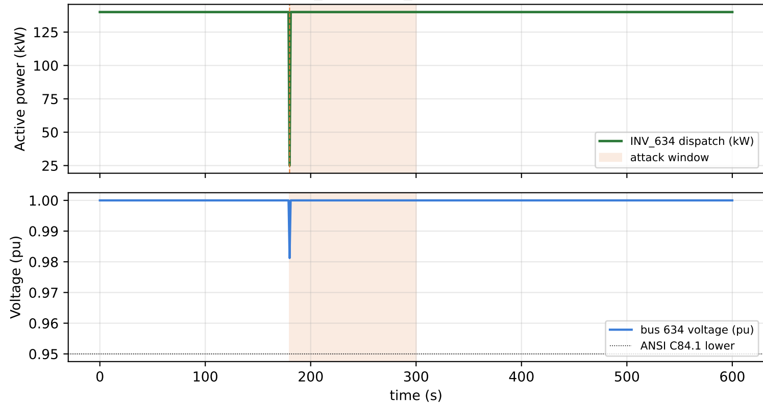
Case study: ieee13_command_spoof --- DER-SecAgent timeline
