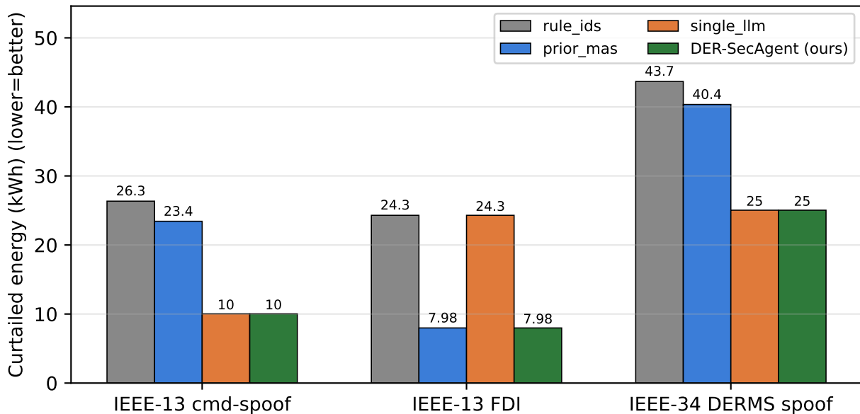
Curtailed energy (kWh) by scenario × detector (mean over 5 seeds)
