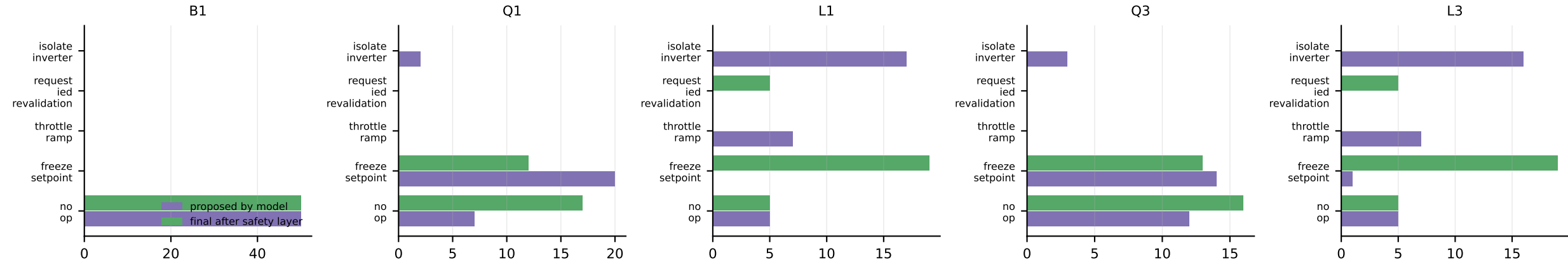
Model proposal vs. executed action (real QLoRA in the loop)
