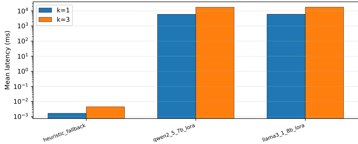
LLM latency by backend × K (bars: ms; annotated 'not run' rows)
