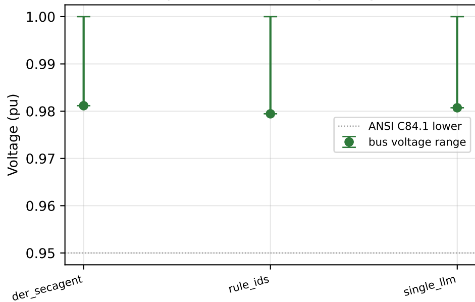
OpenDSS: bus voltage range
