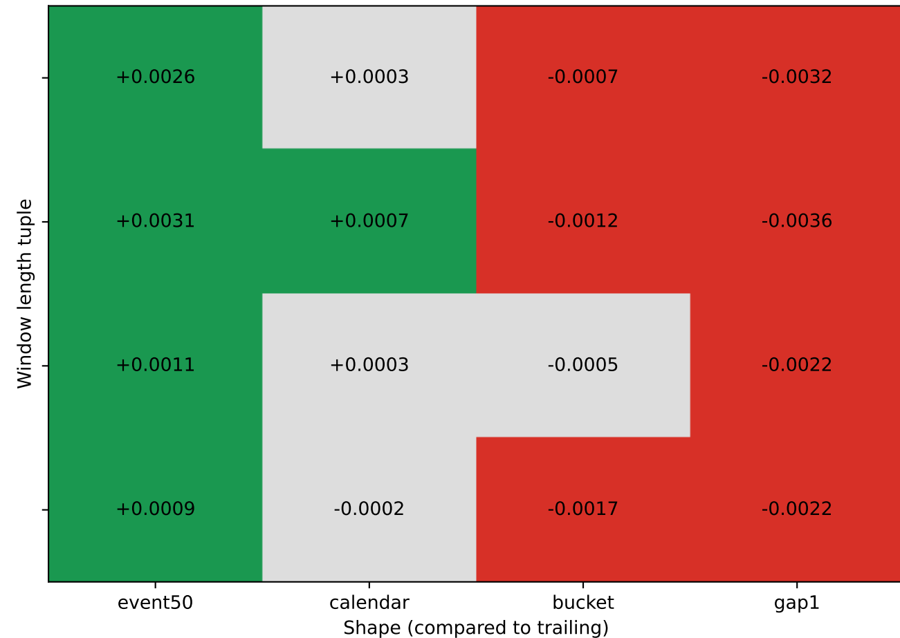
Traffic light: shape effect vs trailing (no TE) Green=better, Red=worse, Gray=unclear (paired DeLong CI, both folds)
