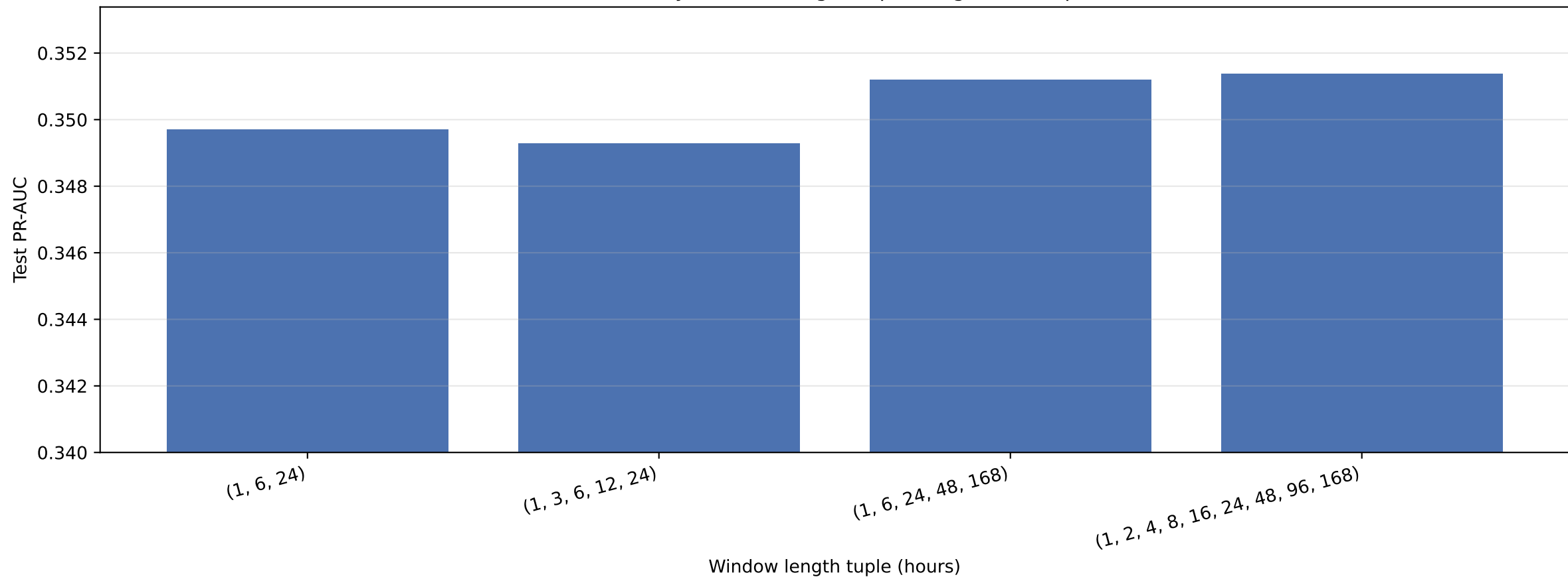
no-TE: Test PR-AUC by window-length tuple (avg over shapes and folds)
