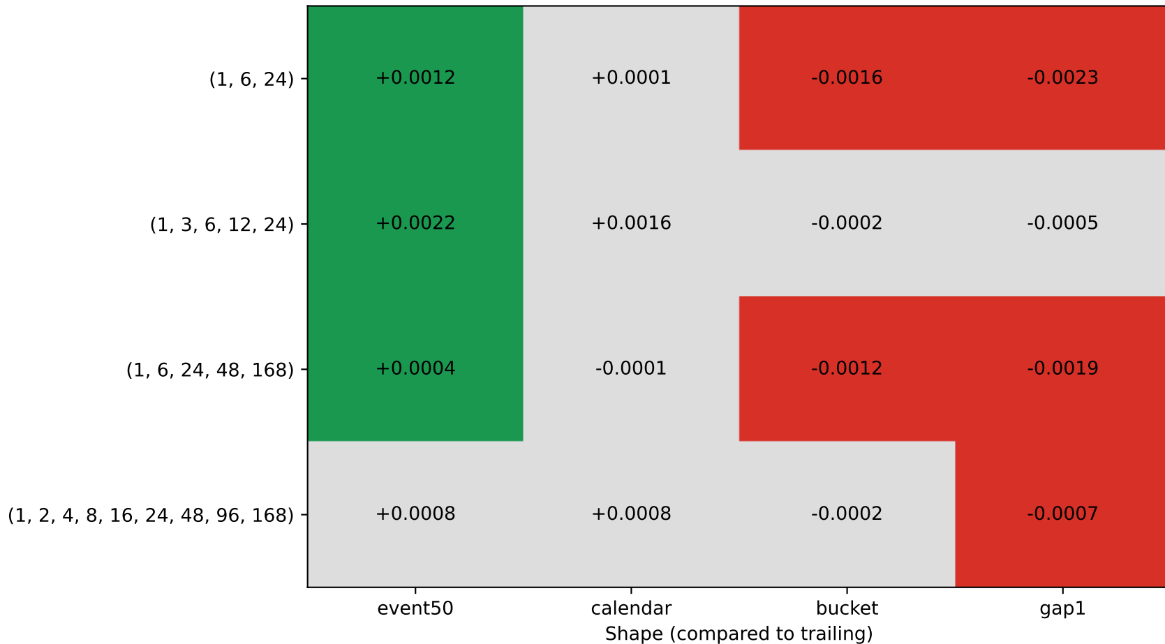
Traffic light: shape effect vs trailing (TE + time-agg) Green=better, Red=worse, Gray=unclear (paired DeLong CI, both folds)
