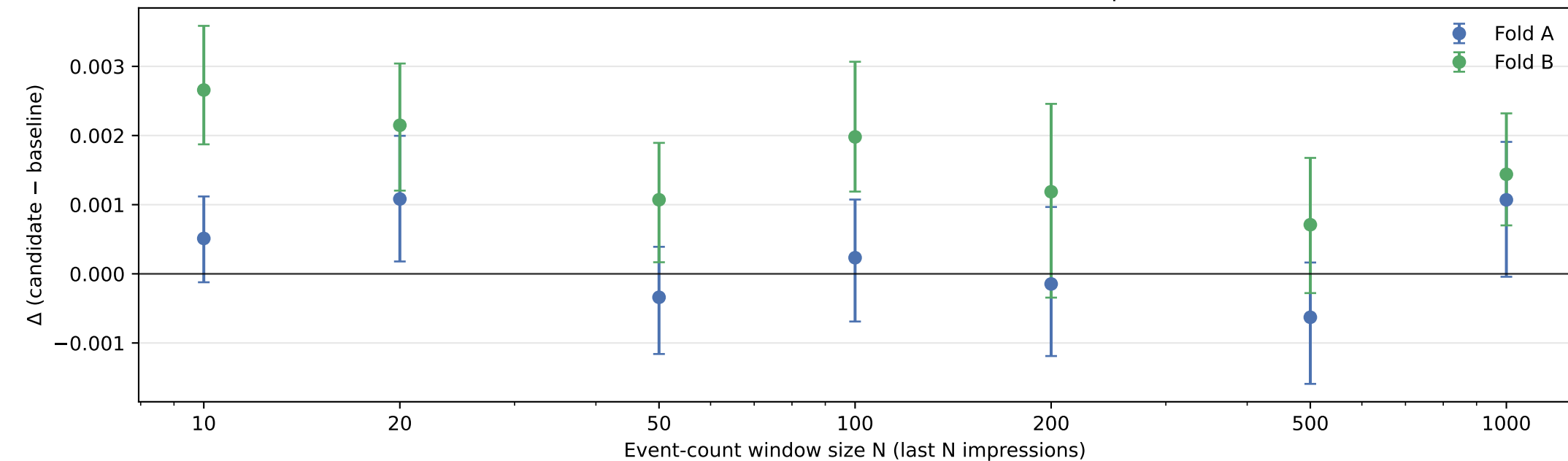
Paired \Delta Test PR-AUC vs baseline (hour-block bootstrap 95% CI)
