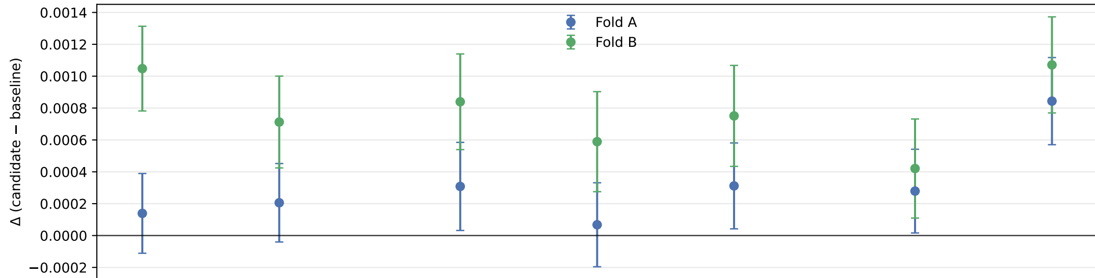
Paired \Delta Test ROC-AUC vs baseline (DeLong 95% CI)
