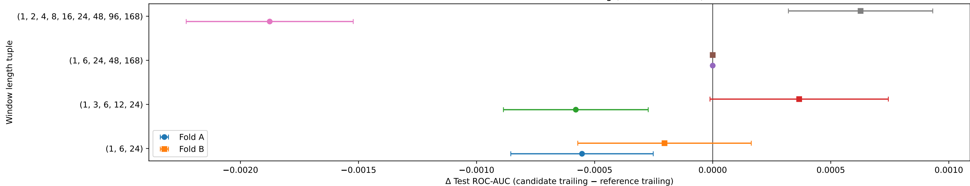
Panel A: Choose window lengths first (trailing only) Test ROC-AUC delta vs reference trailing (1, 6, 24, 48, 168)
