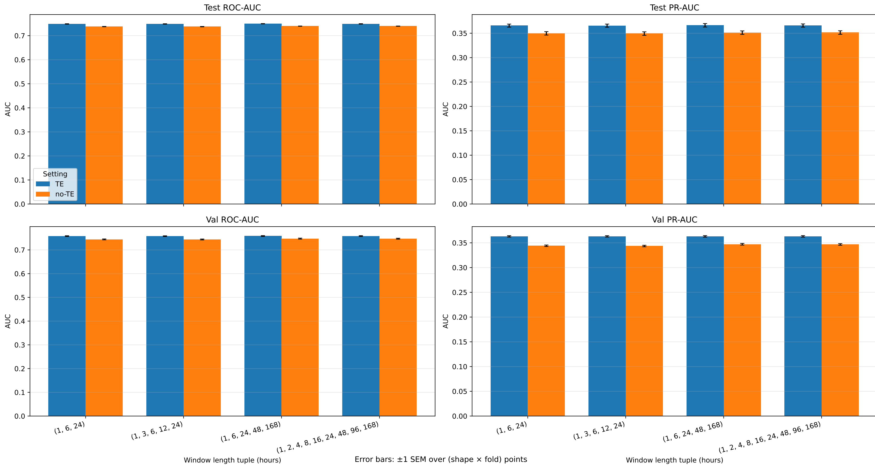
Average performance by window-length tuple (averaged over shapes and folds)
