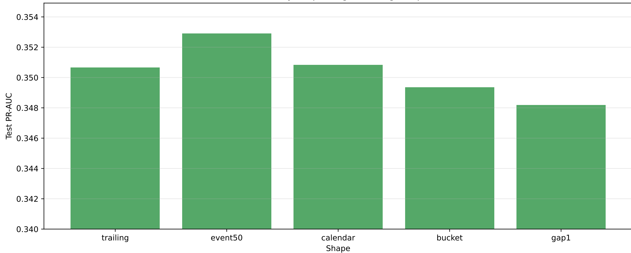
no-TE: Test PR-AUC by shape (avg over length tuples and folds)
