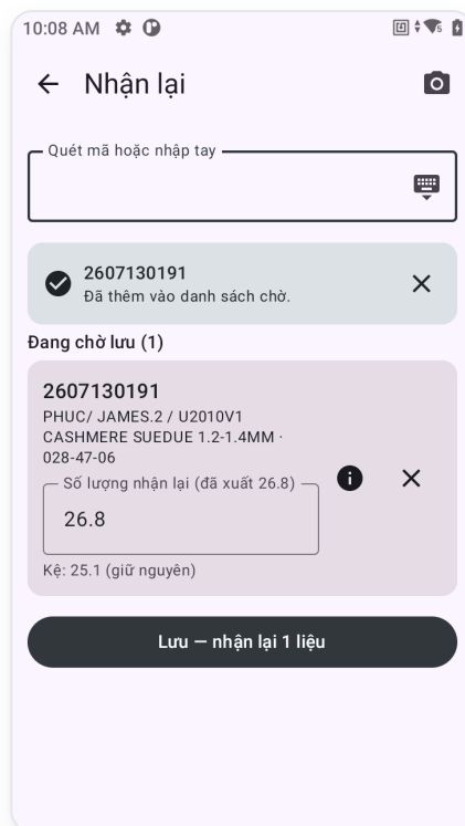
Return — outstanding qty pre-filled
