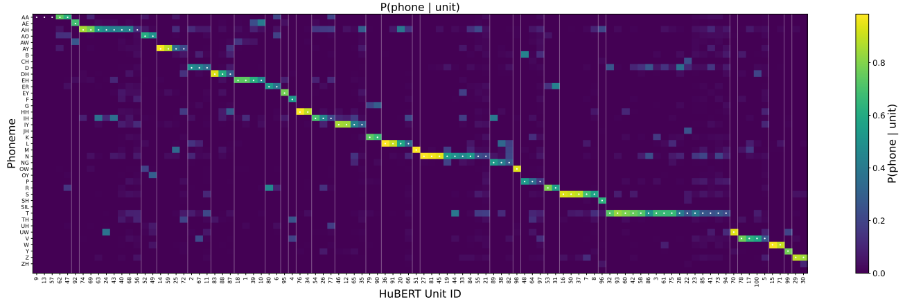
Figure 6: For each HUBERT unit, the phoneme with the highest conditional probability (i.e., \text{argmax}_{\text{PHONE}} P(\text{PHONE} | u) ) is shown. Multiple HUBERT units may map to the same most-probable phoneme p . In such cases, for each phoneme p , we order the corresponding units from left to right by increasing entropy of P(\cdot | u) .
