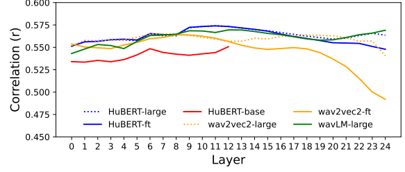
Figure 3: Layer-wise correlation ( r ) between \mathcal{B} and \mathcal{H} across different self-supervised speech models. A simple linear mapping is used to predict \mathcal{B} from \mathcal{H} .
