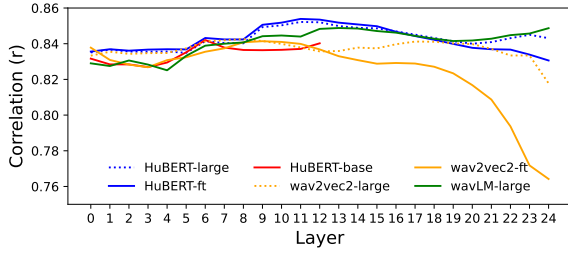
Figure 2: Layer-wise correlation ( r ) between \mathbb{D}(\mathcal{E}) and \mathcal{H} across different self-supervised speech models. A simple linear mapping is used to predict \mathbb{D}(\mathcal{E}) from \mathcal{H} .
