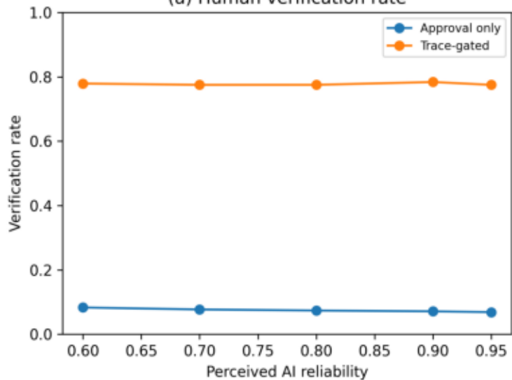
(a) Human verification rate
