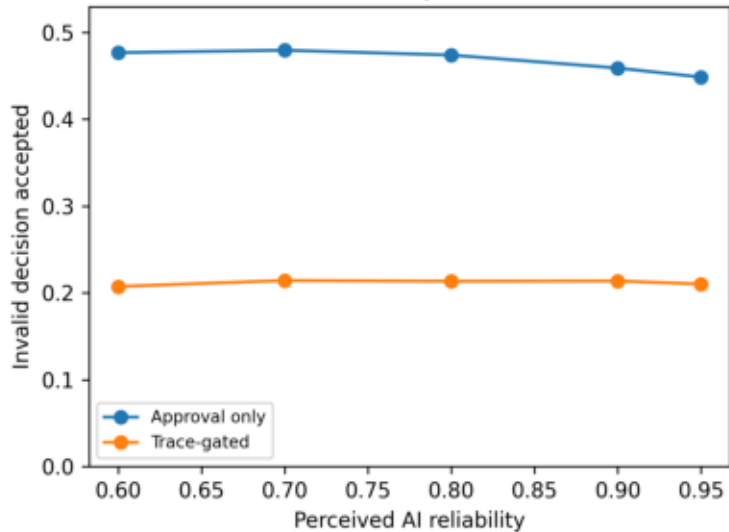
(b) False acceptance rate
