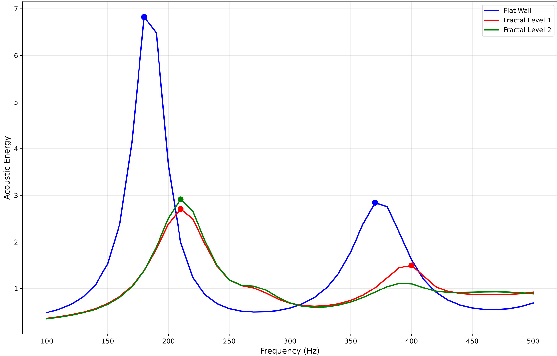
Acoustic Energy vs Frequency for Different Fully Absorbent Wall Shapes
