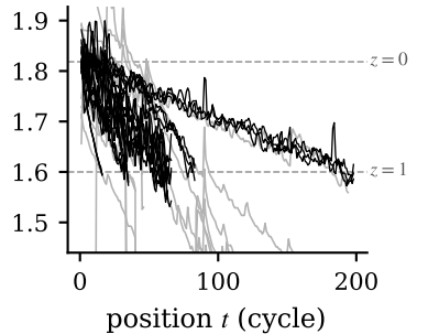
NASA PCoE (18 measured units)
