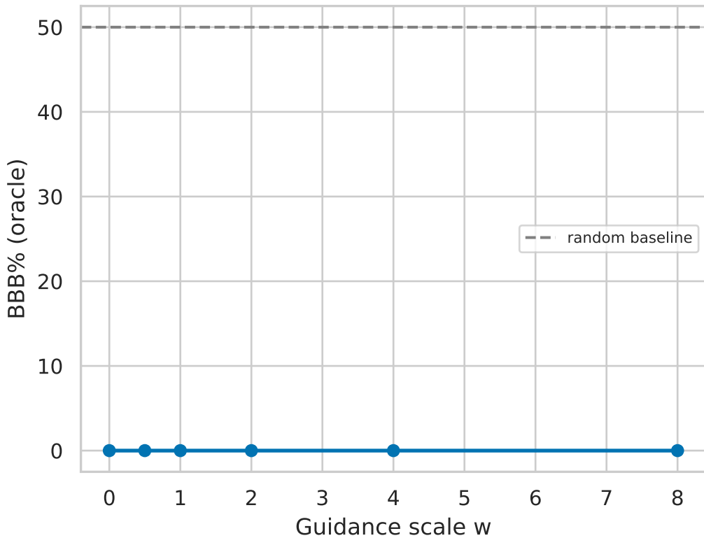
Classifier-free guidance controllability
