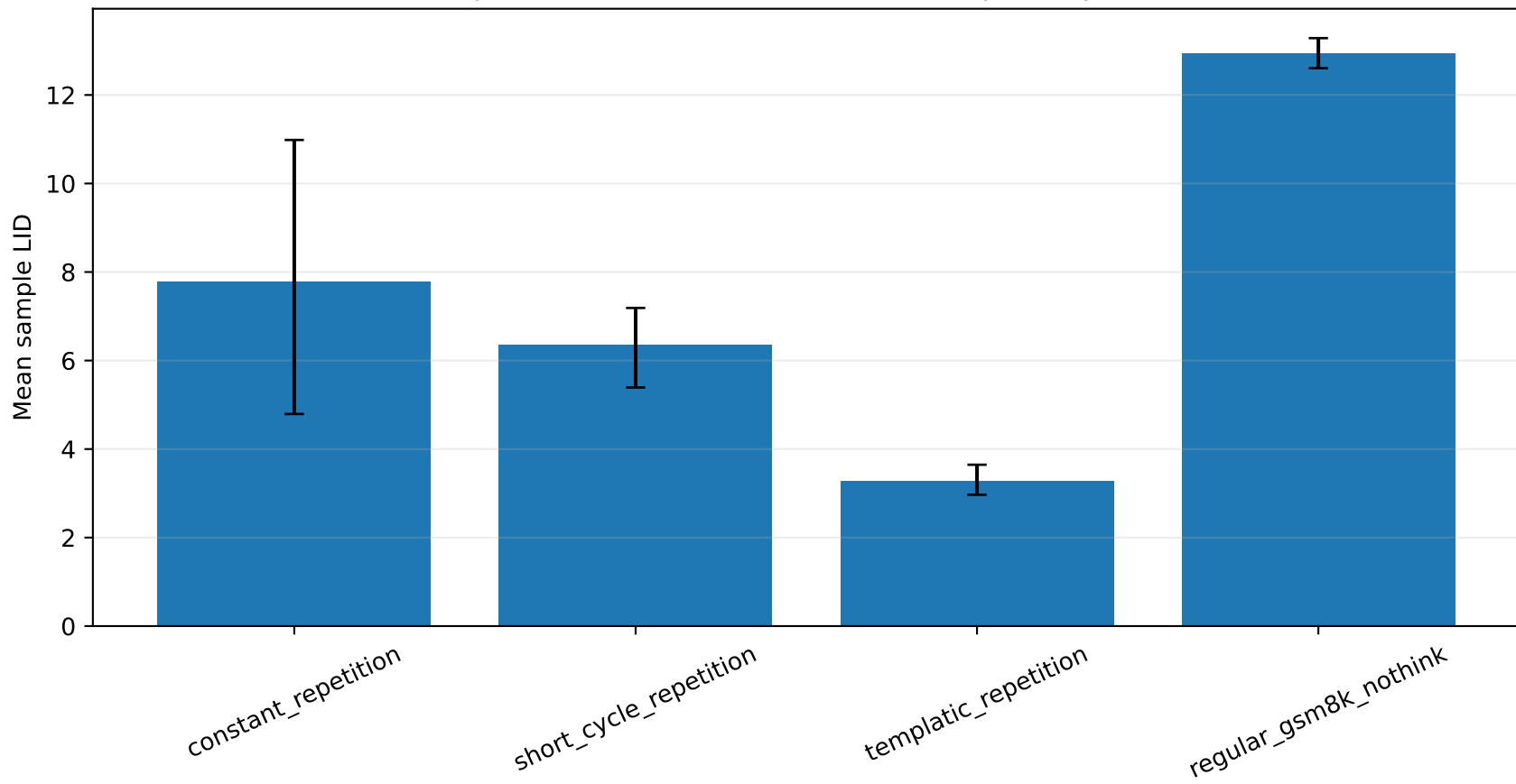
Experiment A mean LID with bootstrap CI, layer 20
