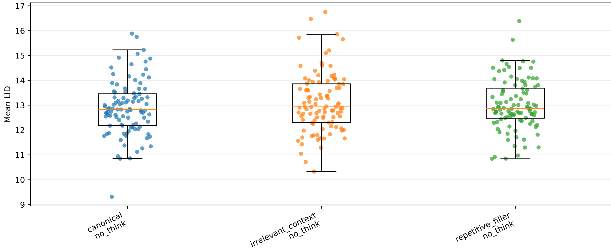
Experiment B answer LID, layer 20
