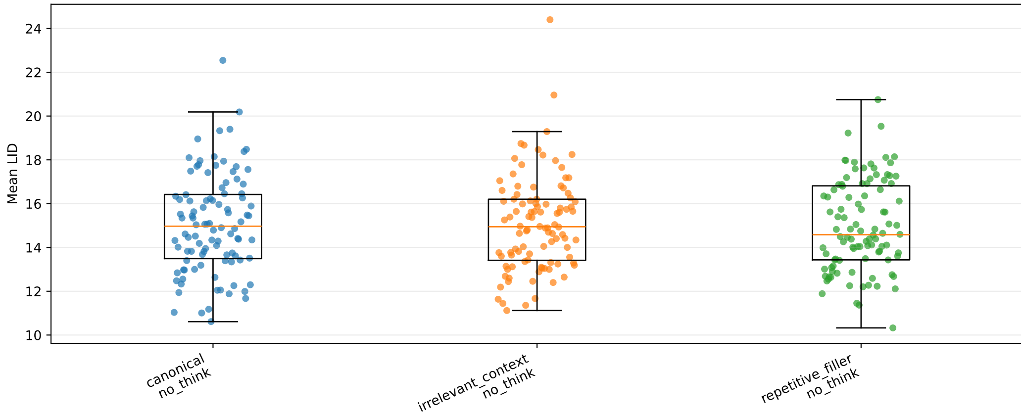
Experiment B answer LID, layer 6
