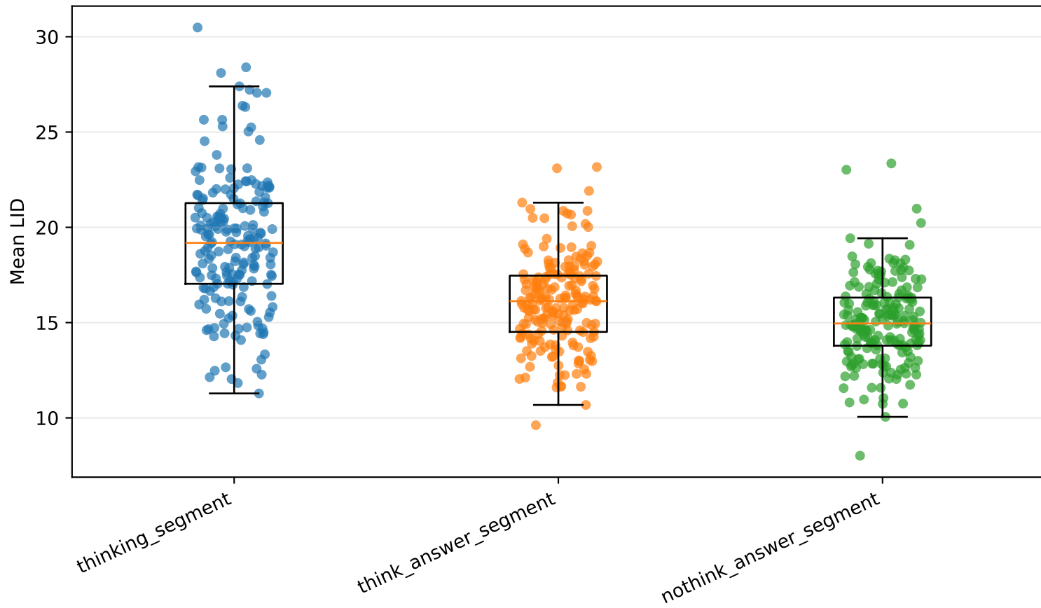
Experiment C segment LID, layer 6
