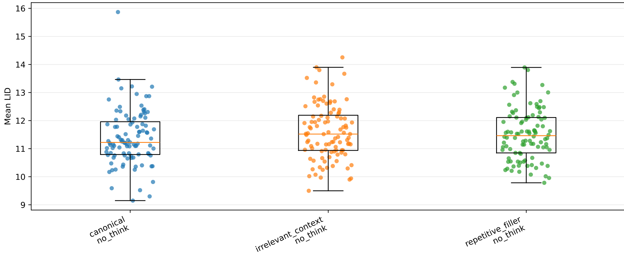
Experiment B answer LID, layer 13
