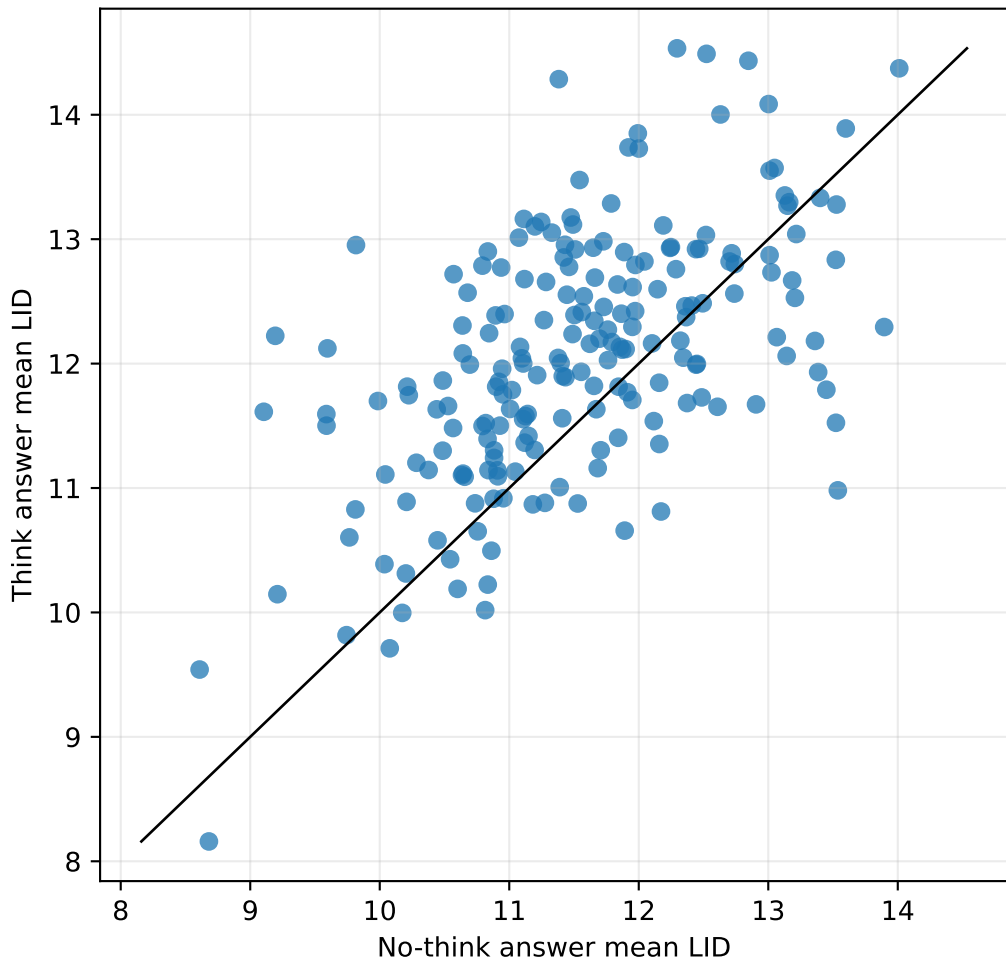
Experiment C paired answer LID, layer 13
