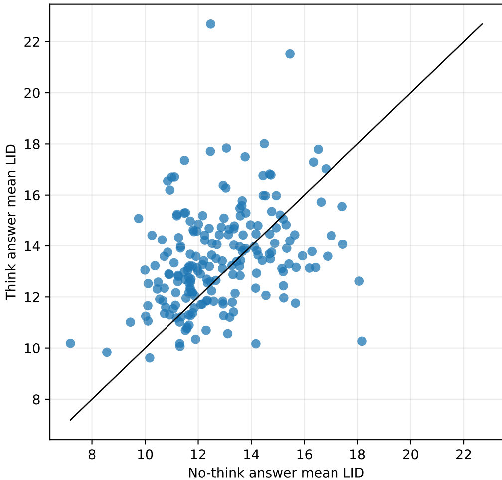
Experiment C paired answer LID, layer 6
