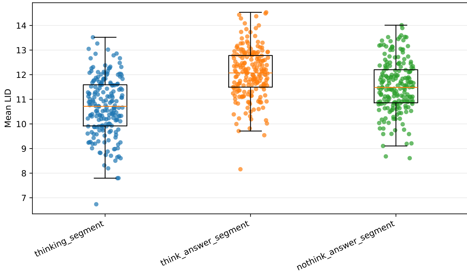
Experiment C segment LID, layer 13
