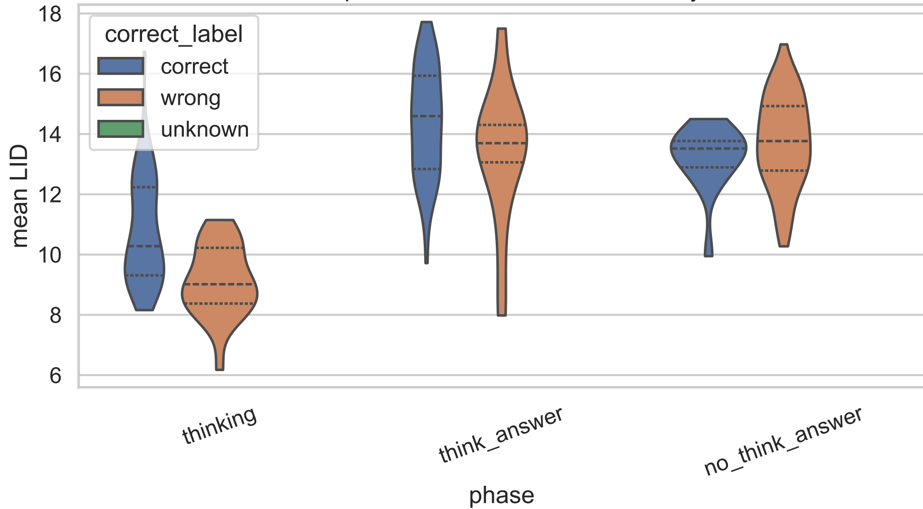
1.7B Exp C correctness-stratified LID, layer 6
