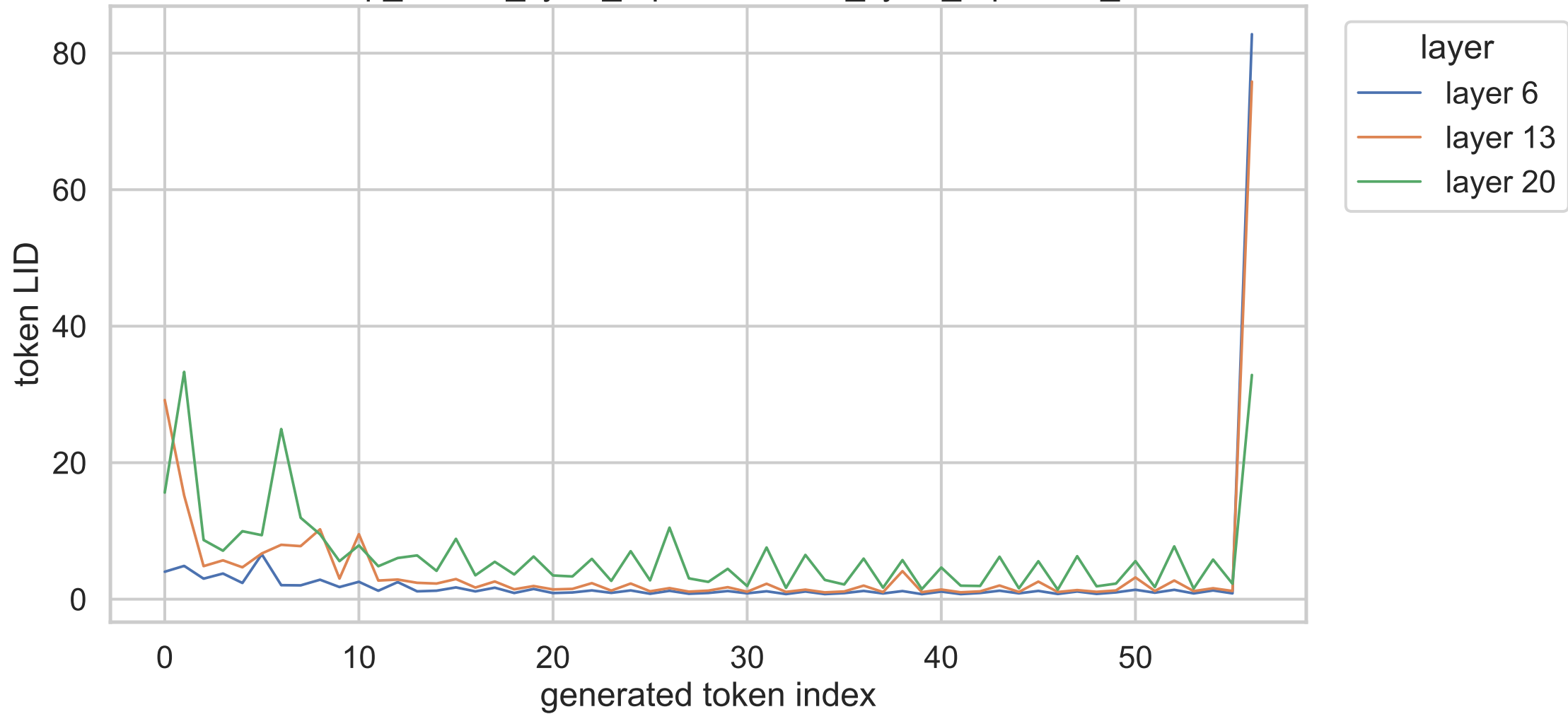
14B exp_a short_cycle_repetition short_cycle_repetition_03
