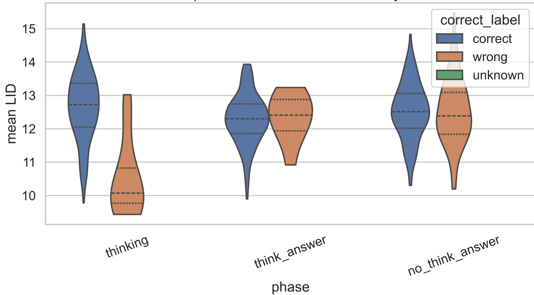
14B Exp C correctness-stratified LID, layer 20
