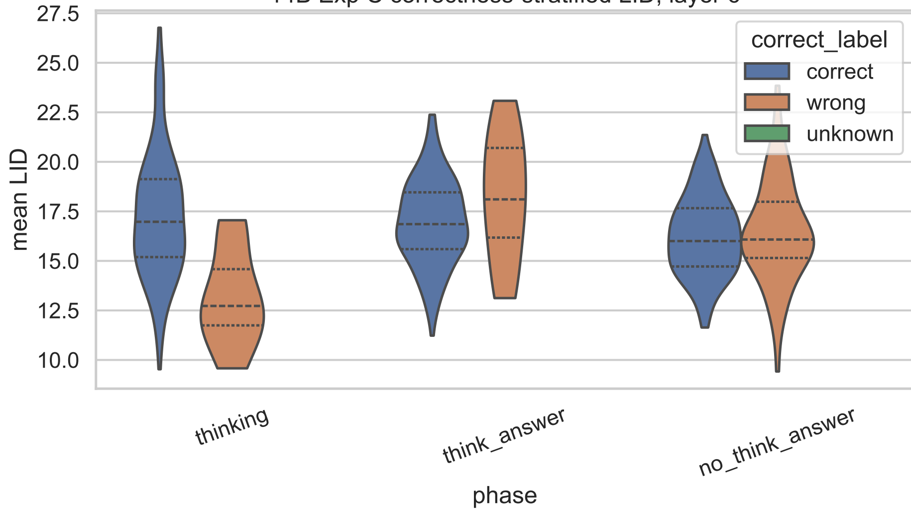
14B Exp C correctness-stratified LID, layer 6
