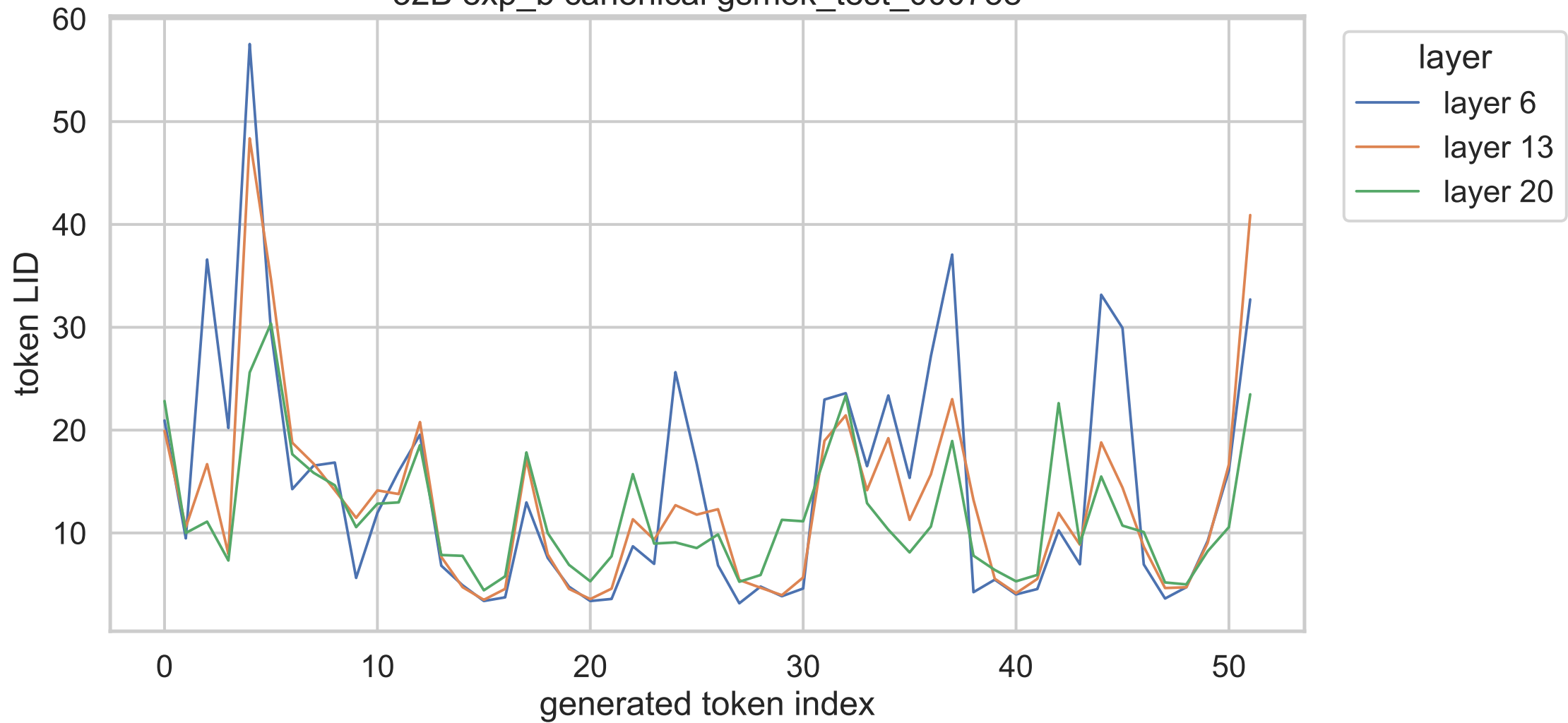
32B exp_b canonical gsm8k_test_000758
