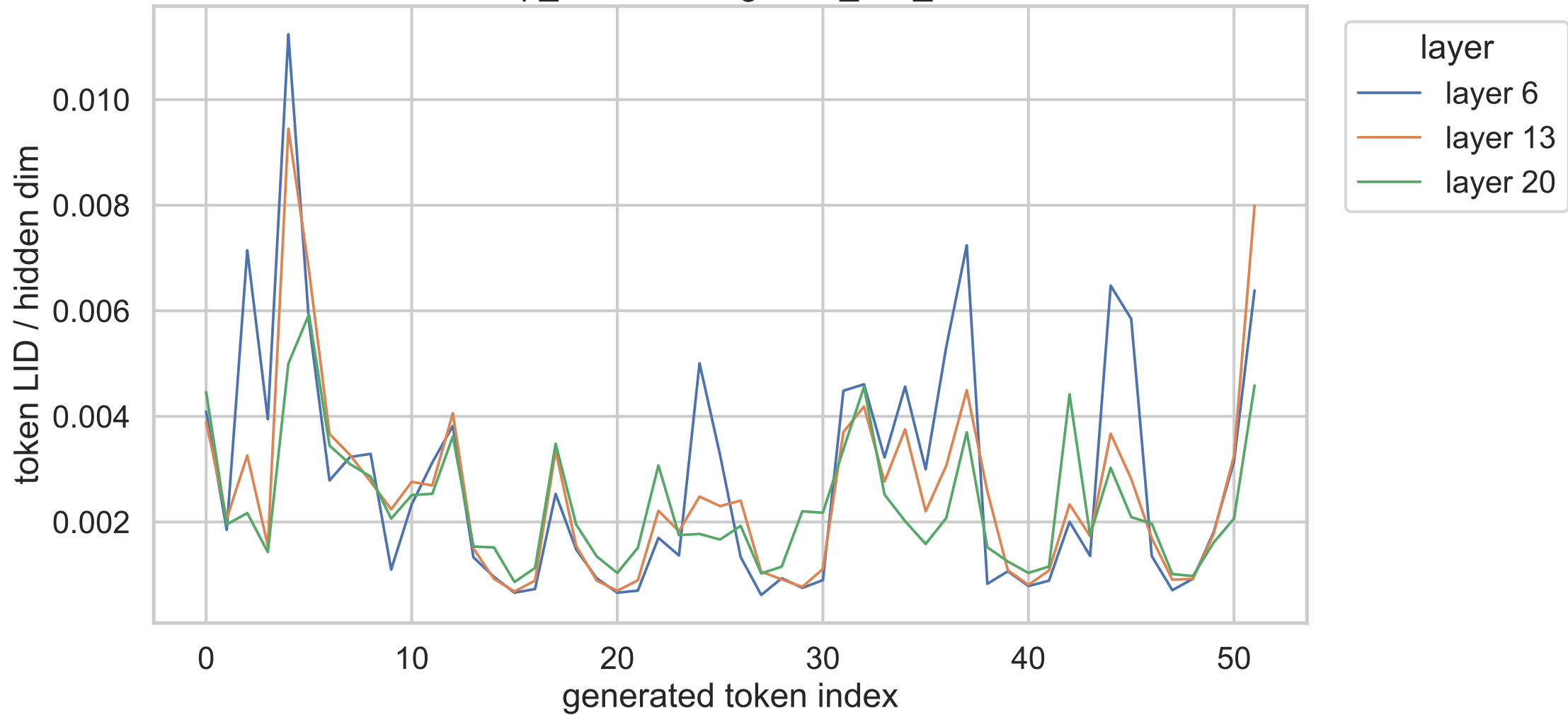
32B exp_b canonical gsm8k_test_000758
