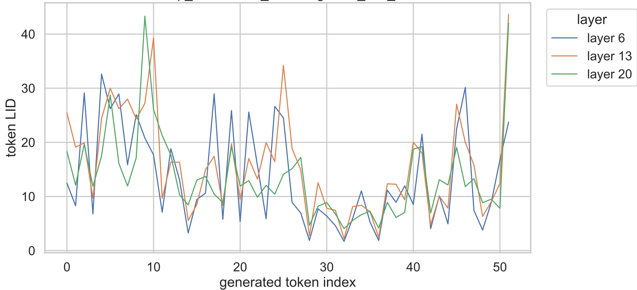
32B exp_b irrelevant_context gsm8k_test_000075
