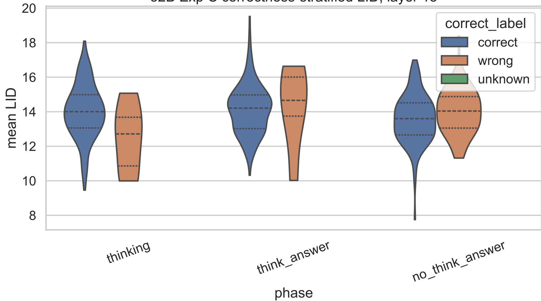
32B Exp C correctness-stratified LID, layer 13
